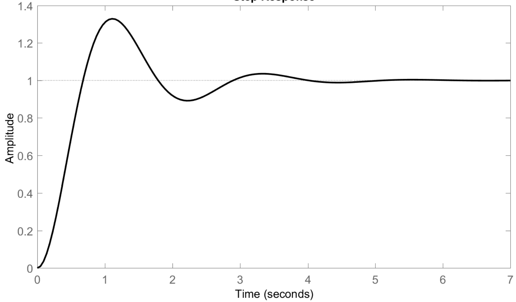
Step Response
